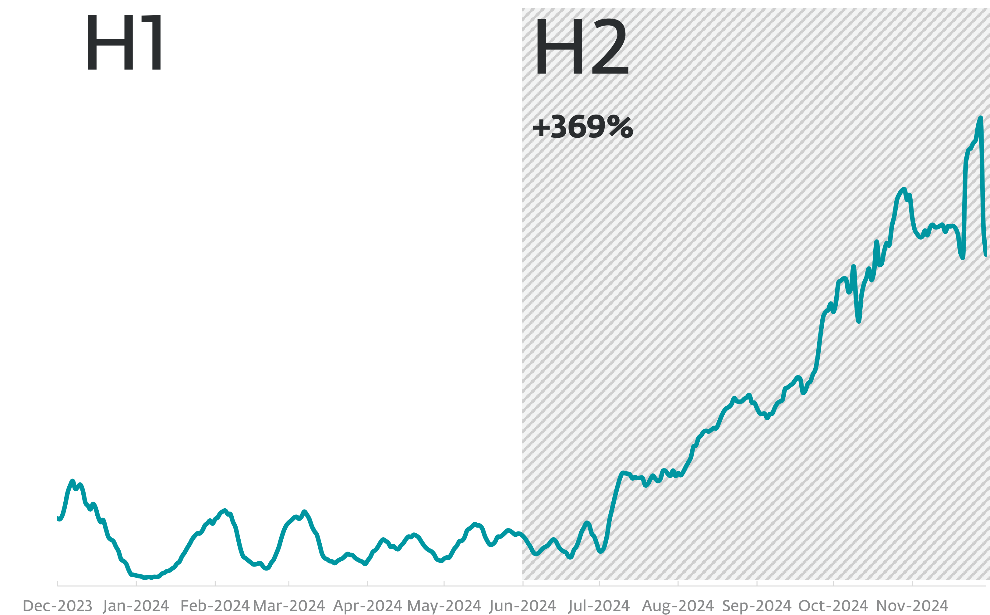
Lumma Stealer detection trend in H1 and H2 2024, seven-day moving average
