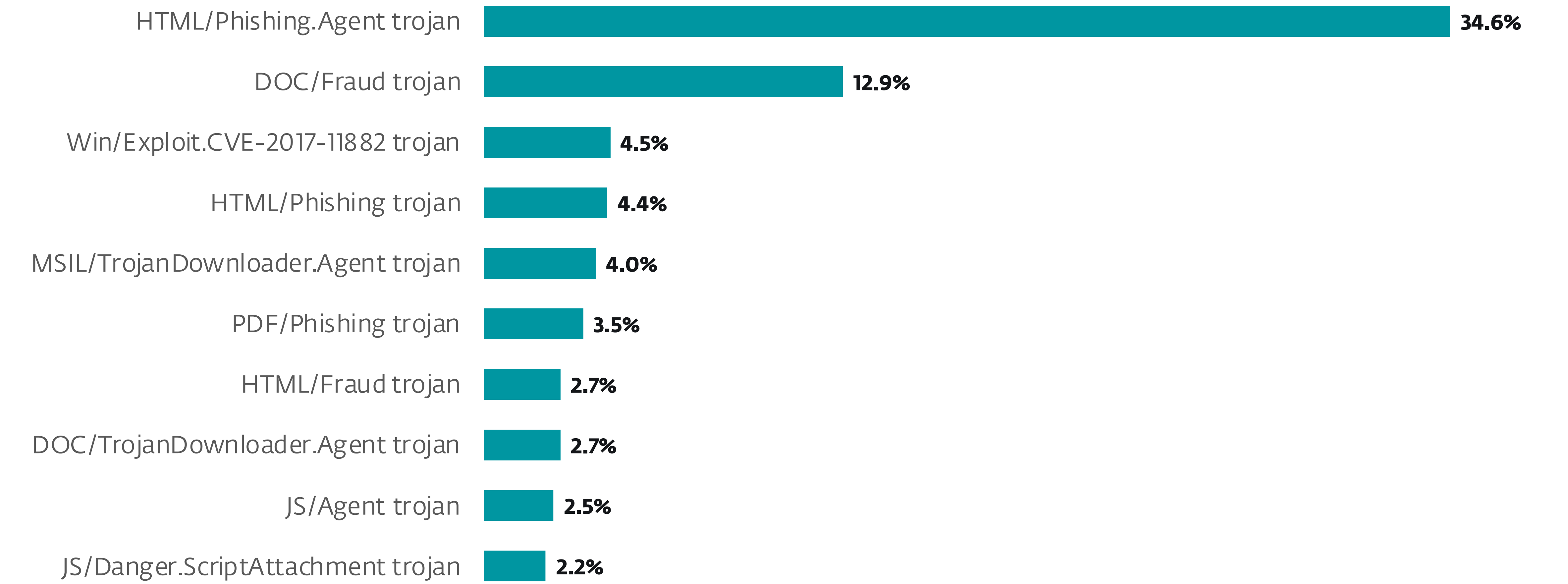
Top 10 threats detected in emails in H2 2024
