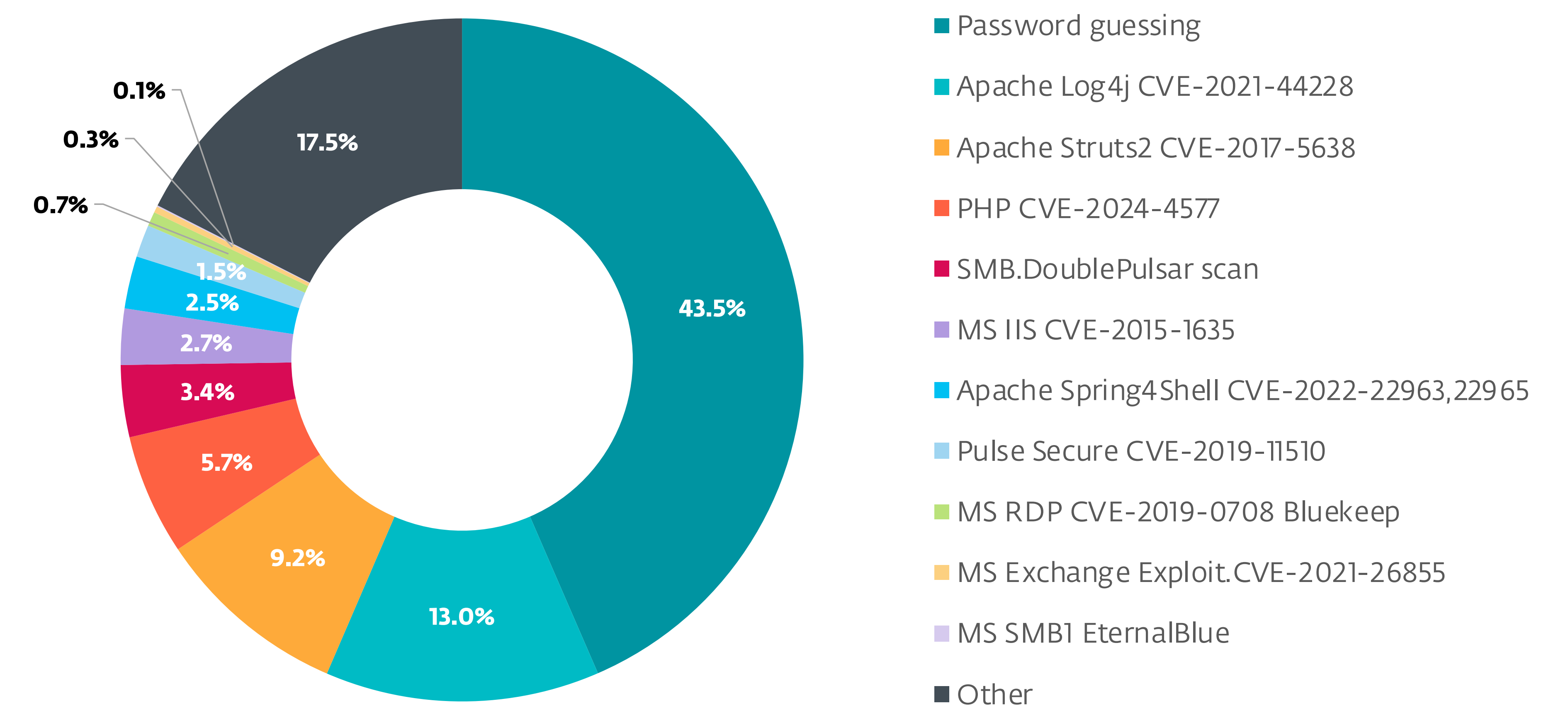
External network intrusion vectors reported by unique clients in H2 2024
