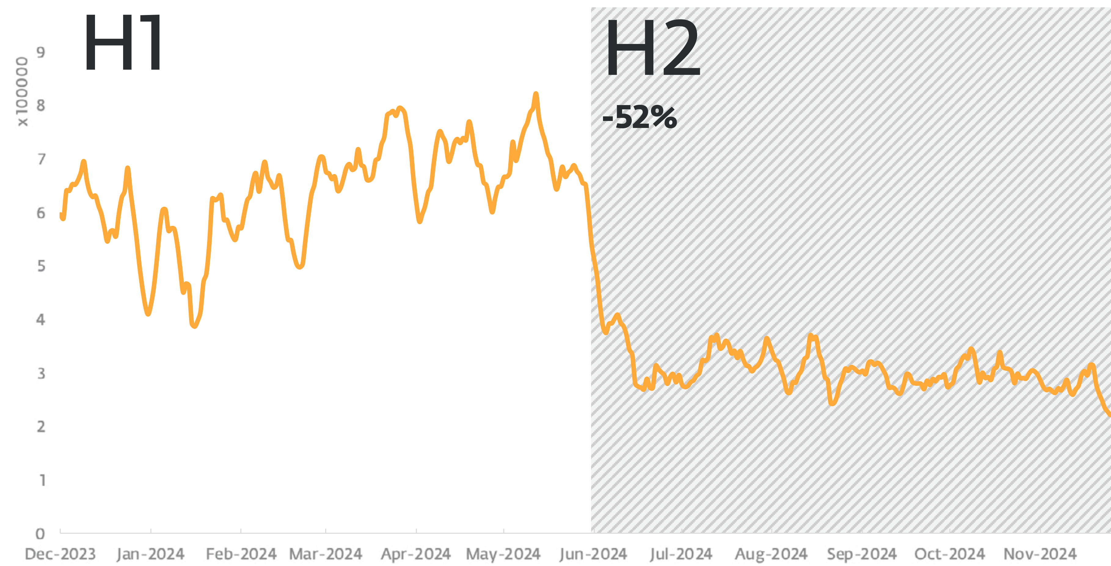
Detection trend of Log4Shell exploitation attempts in H1 2024 and H2 2024, seven-day moving average
